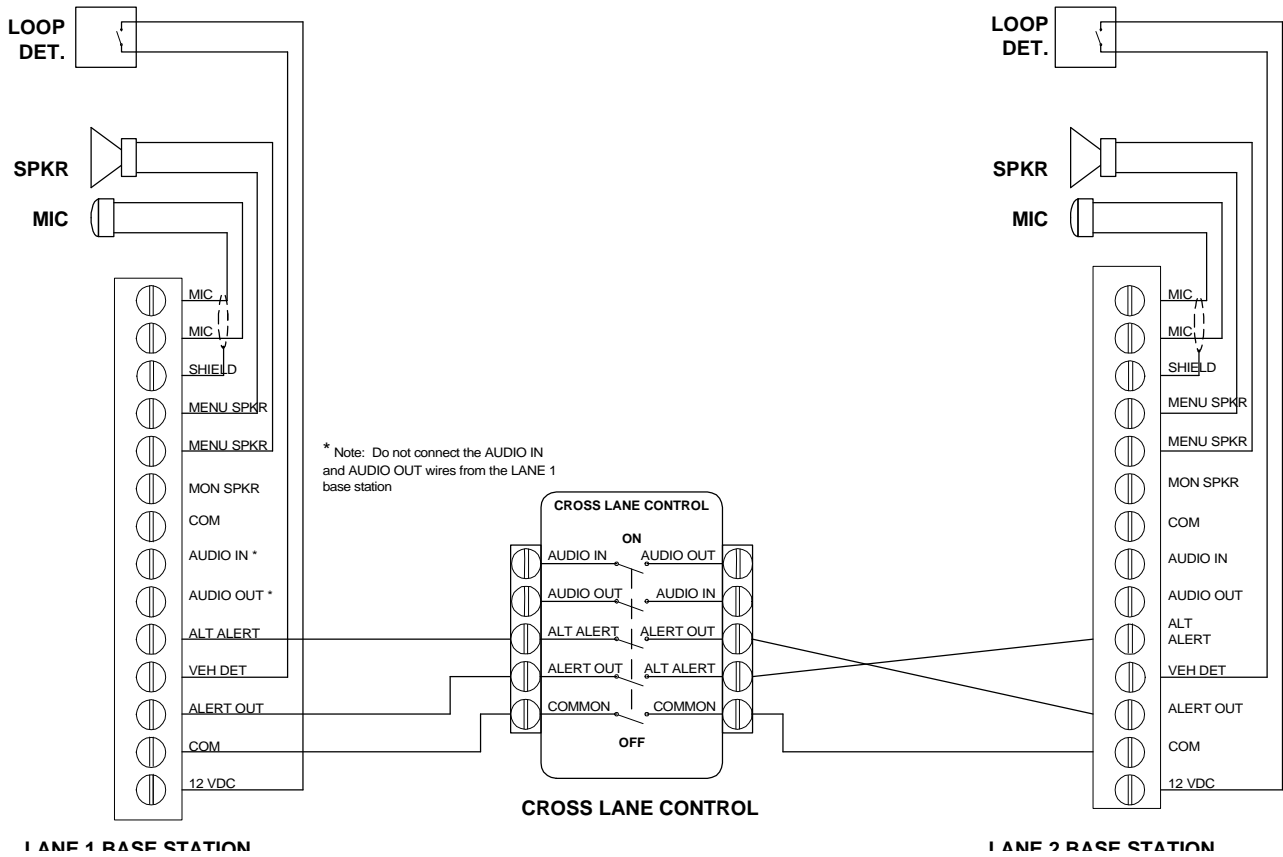
Figure 12. Cross-Lane Wiring Diagram
