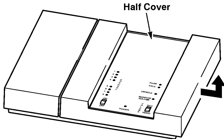
Figure 13. Removing the Half-Cover from the Base Station
