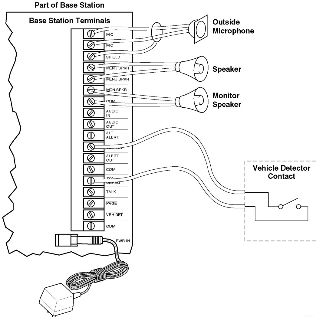
Figure 6. Direct Base Station-to-Component Connections
