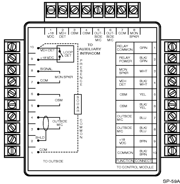
Figure 5. Interconnect Module
