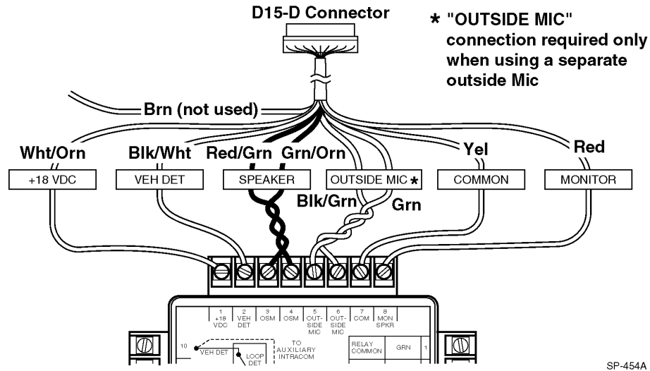
Figure 9. D-15D (M478 DA) Connections
