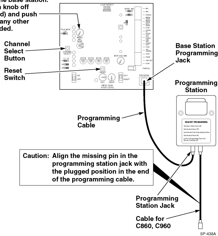
Figure 14. Base Station Circuit Board
