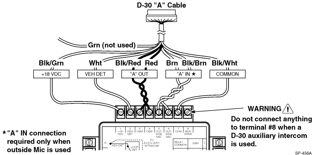
Figure 11. D-30 Connections
