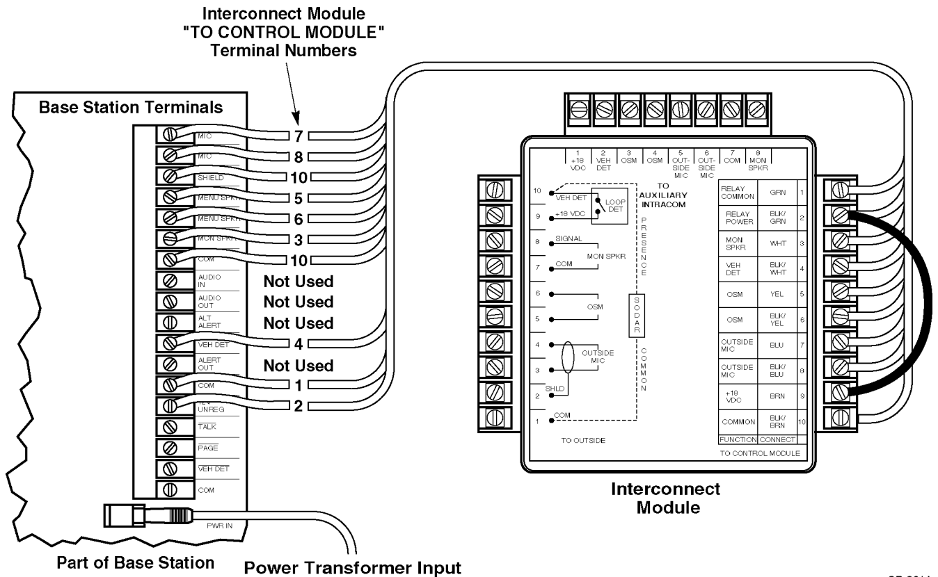
Figure 7. Base Station – Interconnect Module Connections
