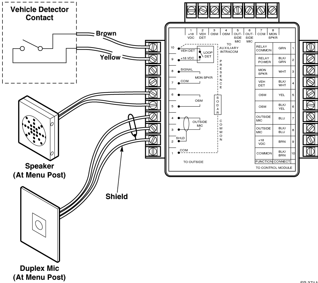
Figure 8. Connecting Components to the Interconnect Module
