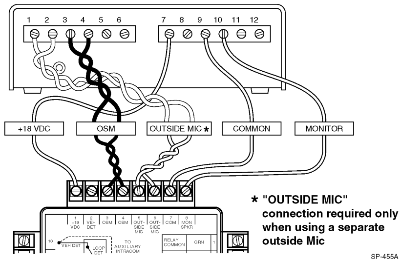
Figure 10. D-15B and D-15C (M478 BA and CA) Connections
