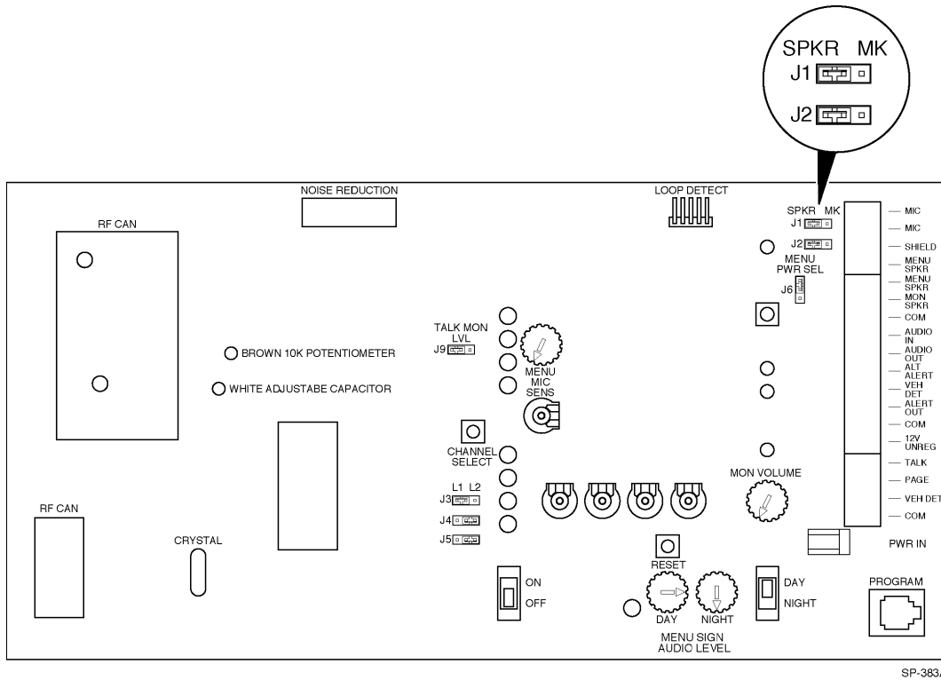
Figure 15. Base Station Circuit Board
